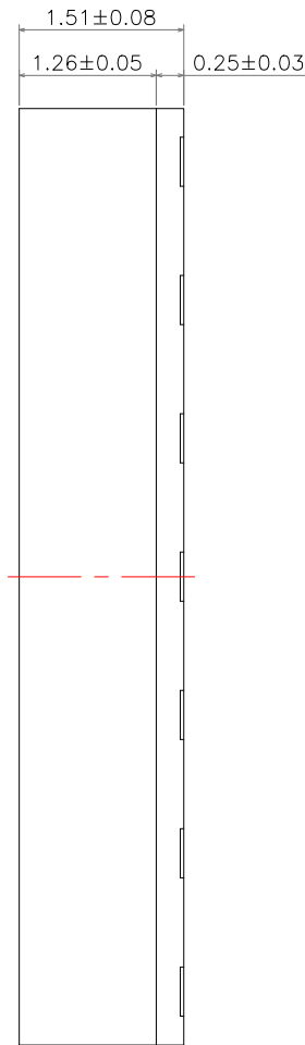
SIDE VIEW
